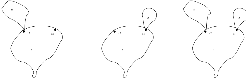
FIGURE 4. Exemple of the third case above. The trees are respectively \mathbf{t}_1 , \mathbf{t}_2 , \mathbf{t}_1 \cup \mathbf{t}_2 .
