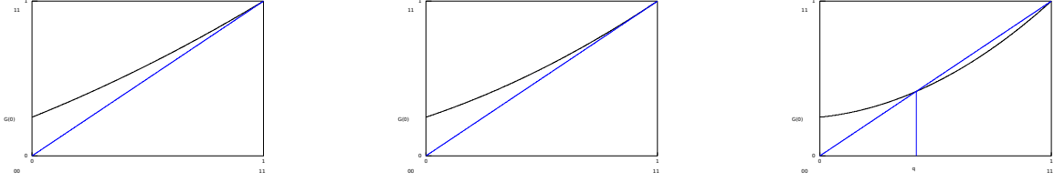
FIGURE 2. Generating function in the sub-critical (left), critical (middle) and super-critical (right) cases.
